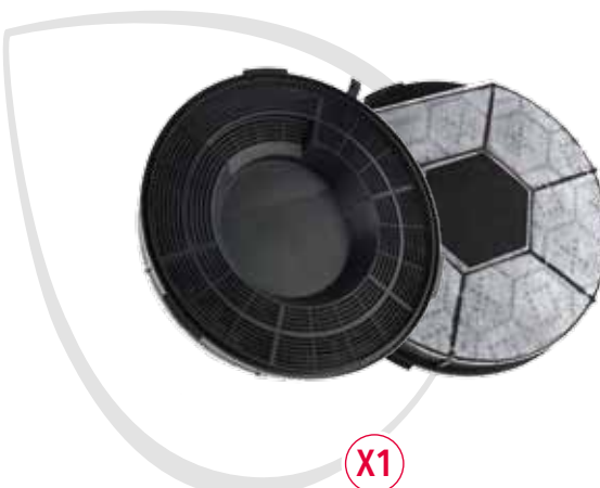
KFC6904 (CP028) 35602047 EAN 8016361971202 Ø240x32mm; 410gr - Tipo 028
